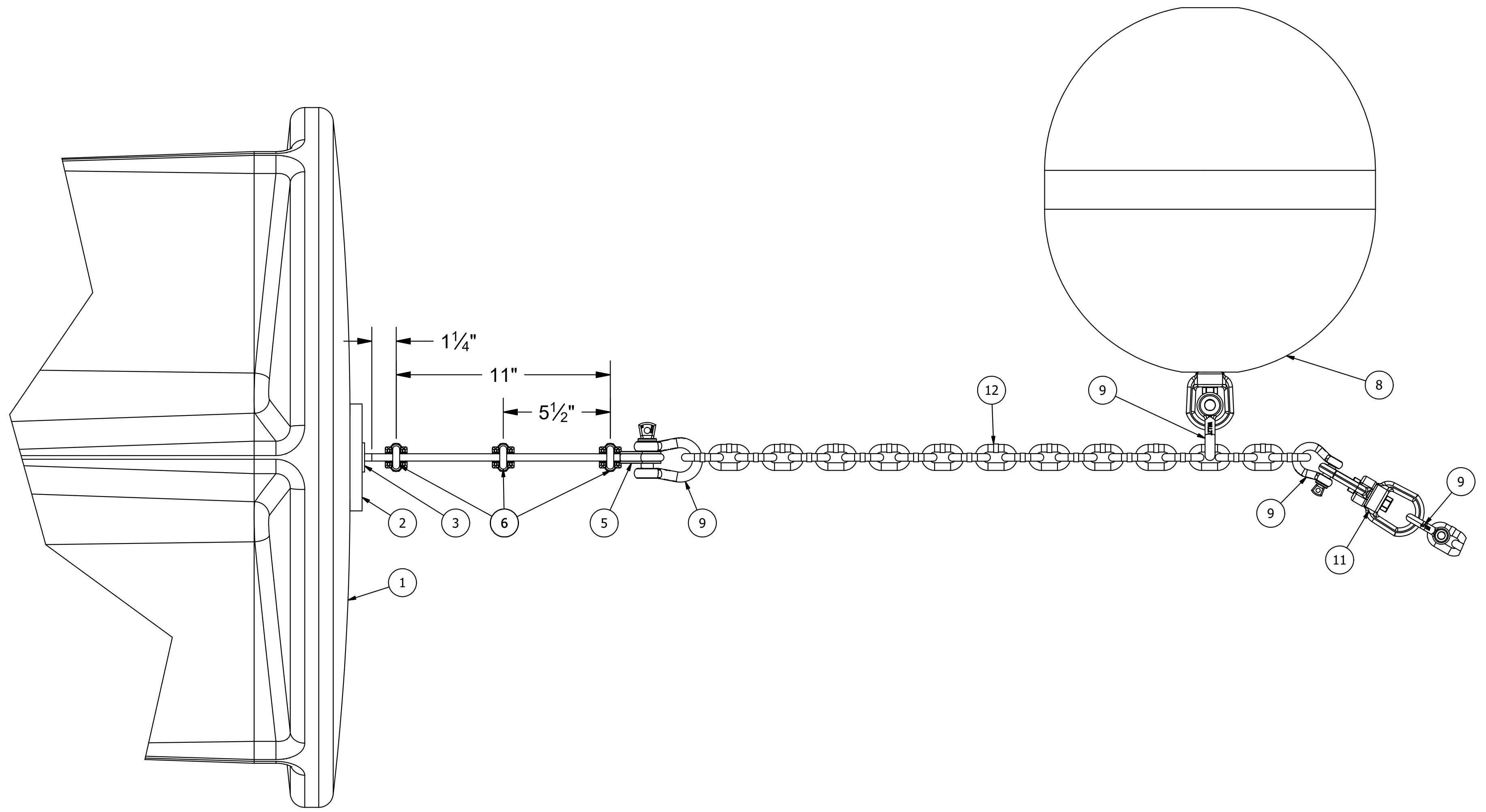
DETAIL A
