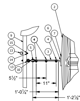
DETAIL F
