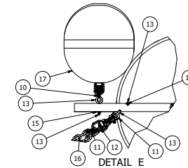
DETAIL E
